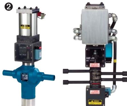
Burner & Igniter Safety Shutoff Valve
